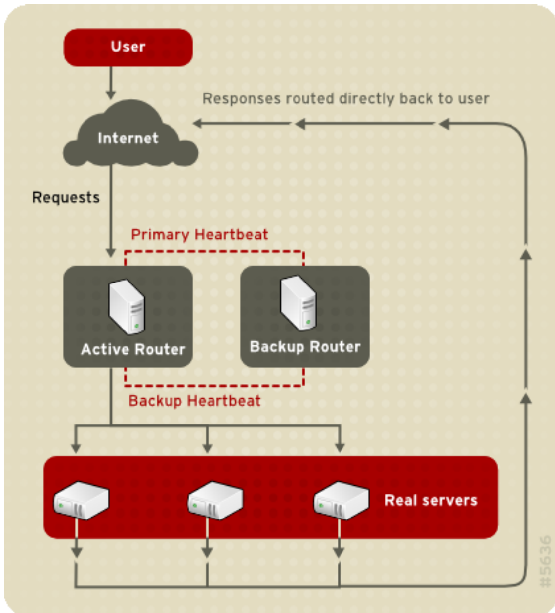
Figure 1.23. LVS Implemented with Direct Routing
