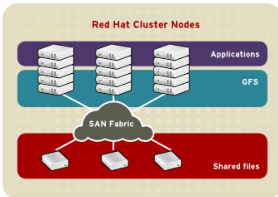
Figure 1.11. GFS with a SAN
