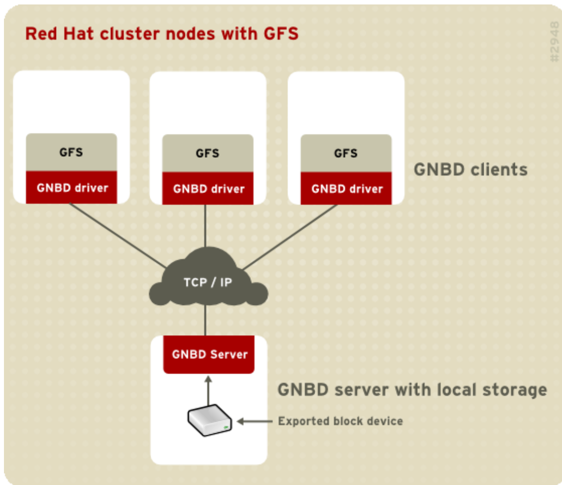
Figure 1.18. GNBD Overview
